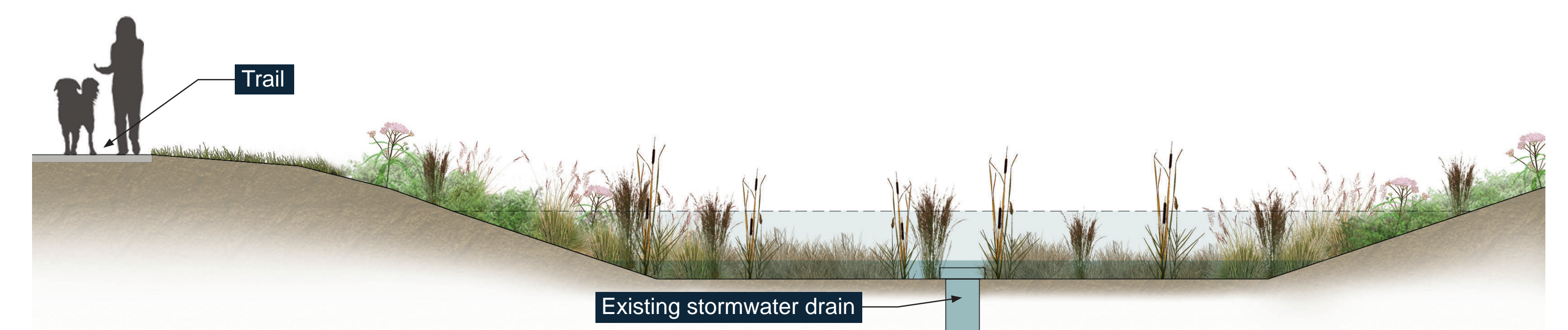
D. Proposed bioretention section
